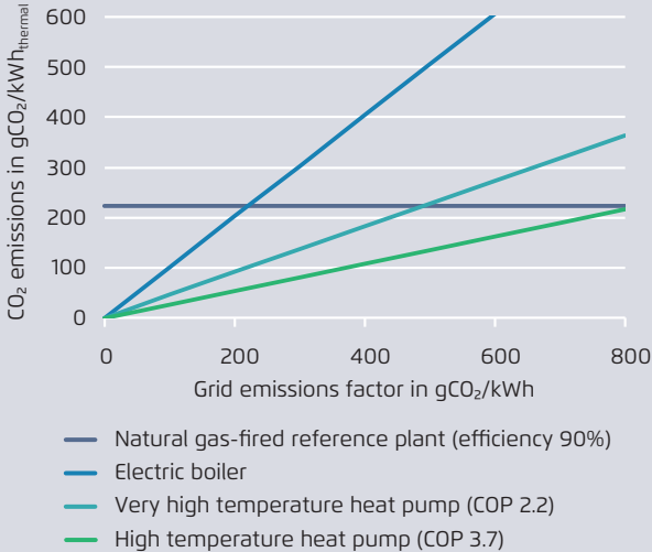
a) CO 2 emissions of electricity-based technology options compared to a natural gas-fired steam boiler
