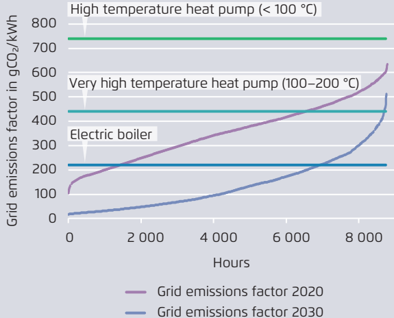
b) Grid emissions factors for 2020 and 2030 and thresholds below which operation is ecologically beneficial
