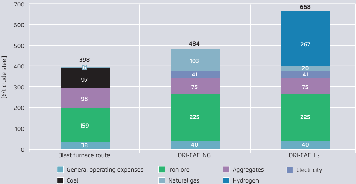
Breakdown of relevant OPEX cost blocks by route (€/t crude steel)
