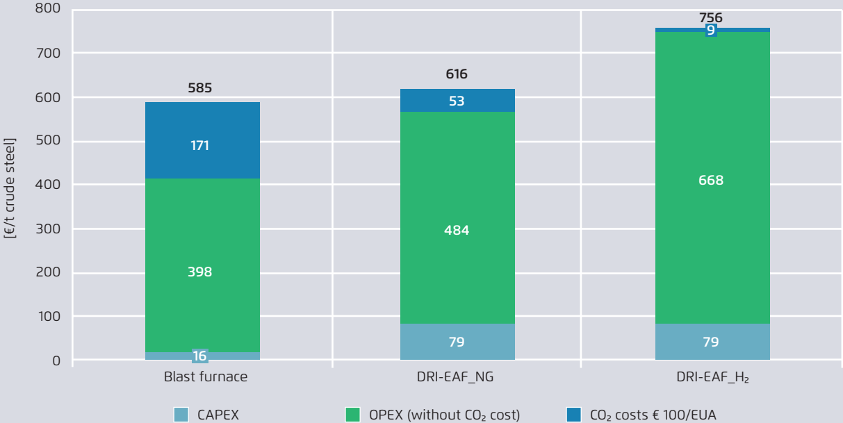
Cost blocks for producing one tonne of crude steel by route (€/t crude steel)
